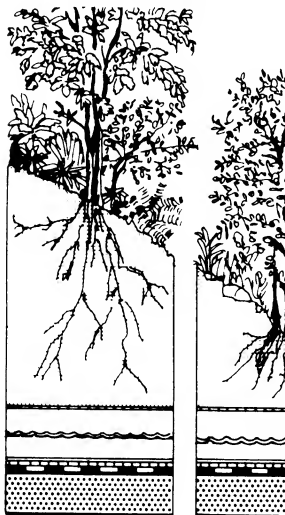
5 Zinco Floraterra roof cultivation system
